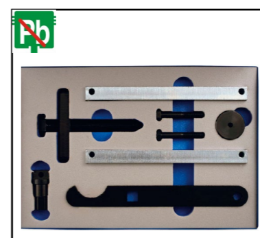
LSR 5147 LASER engine: AC, BC, GB, 1B, 2B capacity: 3.2, 3.5, 4.0, 4.2 year: from 1996 to 2010
