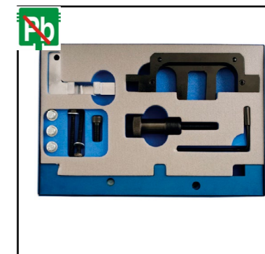
LSR 5095 LASER engine: N40, N45 capacity: 1.6, 2.0 year: from 2002 to 2010
