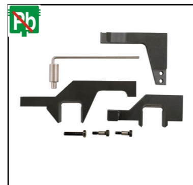
LSR 5149 LASER engine: N12, N14, EP3, EP6, 8F, 5F capacity: 1.4, 1.6 year: from 2006
