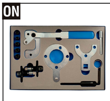
LSR 4773 LASER engine: 169A1.000, F13DTE5, Z13DT capacity: 1.3 year: from 2003 to 2015
