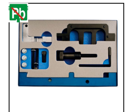
LSR 6561 LASER engine: YSKD, UEJB, HXDA, DHA, FHD, HWDA capacity: 1.25-1.6 16V year: from 1996 to 2010
