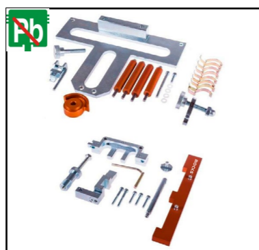
OK-02.3020 ROCKS engine: N42, N46 capacity: 1.8, 2.0 year: from 2001 to 2014
