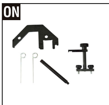
OK-02.3042 ROCKS engine: M47, M57 capacity: 2.0, 2.5, 3.0 year: from 1998 to 2011
