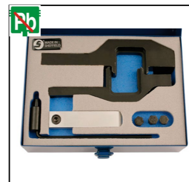
LSR 5148 LASER engine: N14, EP6 capacity: 1.6 year: from 2006 to 2017
