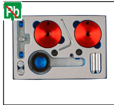
LSR 7323 LASER engine: BCCC, YLCB, YMFA, YNFA capacity: 2.0 year: from 2016
