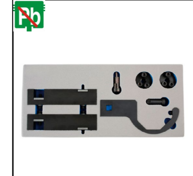
LSR 7051 LASER engine: AJ-126, AJ-133, 508PN/PS capacity: 3.0, 5.0 year: from 2012
