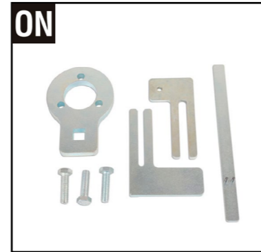
LSR 6301 LASER Balance shaft setting tools for N40, N42, N43, N45, N46, N52
