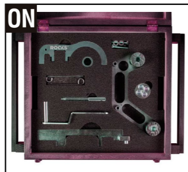
OK-02.3019 ROCKS engine: N47, N57 capacity: 2.0, 3.0 year: from 2007
