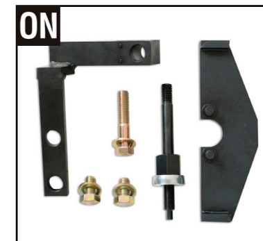
LSR 4408 LASER engine: W10, W11 capacity: 1.4, 1.6 year: from 2001 to 2009
