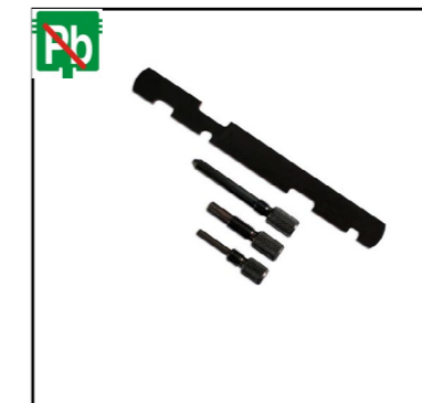
LSR 4347 LASER engine: FUJA, FXJA, HWDA, JQDA capacity: 1.25-2.3 16V year: from 1995 to 2007
